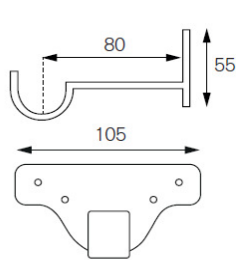
Standard Pole Centre Bracket
