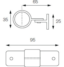
Ceiling Fix Bracket
