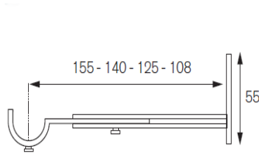
Recess Bracket
