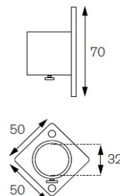
Recess Bracket
