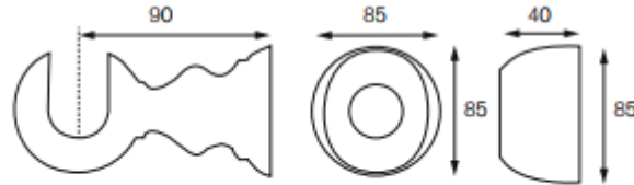
Wooden Cup Bracket
