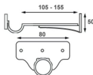
Extension Centre Bracket
