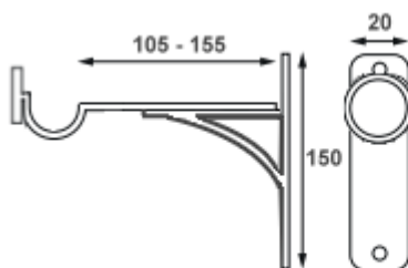
Extension End Bracket
