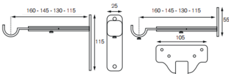
Extension End Bracket
