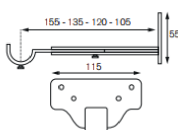
Extension Centre Bracket
