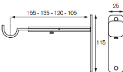
Extension End Bracket
