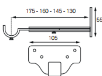
Extension Centre Bracket
