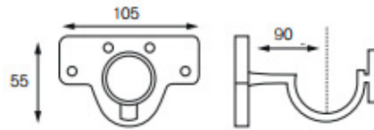
Chrome/Brass Centre Bracket
