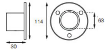
Metal Recess Bracket
